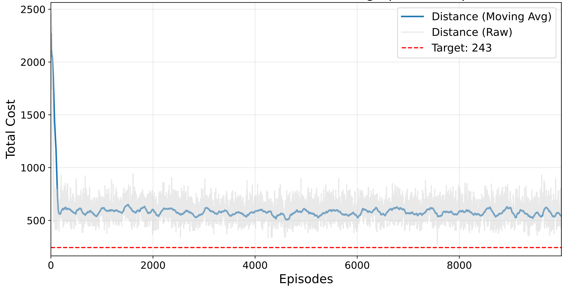
Final Masked AutoRL-SOP Training - prob.42.sop
